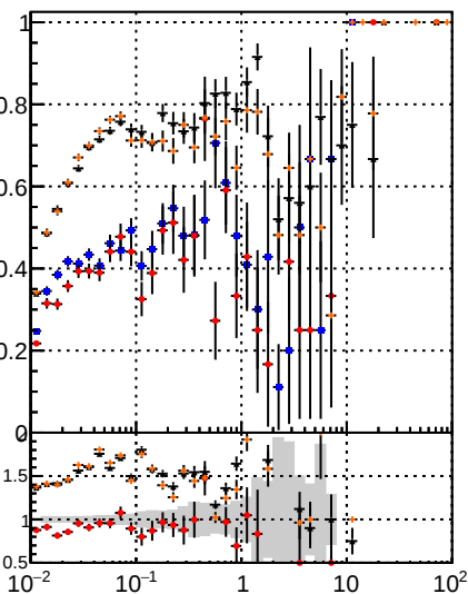
Fake rate vs v Legend: DOM CKE DOM mKEFit DOM BDT DOM mKEFit
