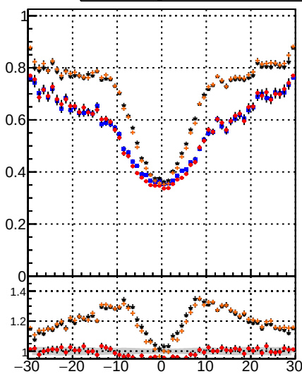
DOM CKE BDT mKEit Fake rate vs vertpos
