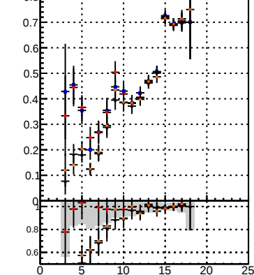
Pileup rate vs layer
