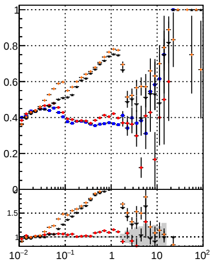
Legend for Fake rate vs vertpos: DOM (blue circles) CKE (orange crosses) BDT (red stars) mKEit (black dots)
