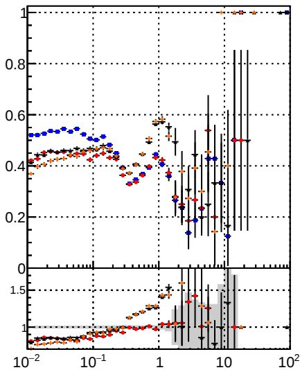
Legend for Fake rate vs vertpos: DOM CKE BDT mKEfit BDT mKEfit
