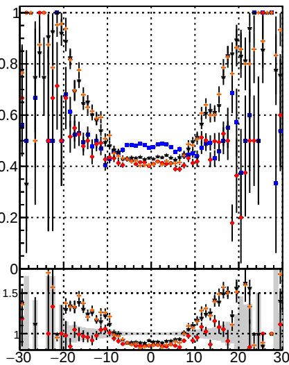
Legend for Fake rate vs vertpos: DOM CKE BDT mKEfit BDT mKEfit
