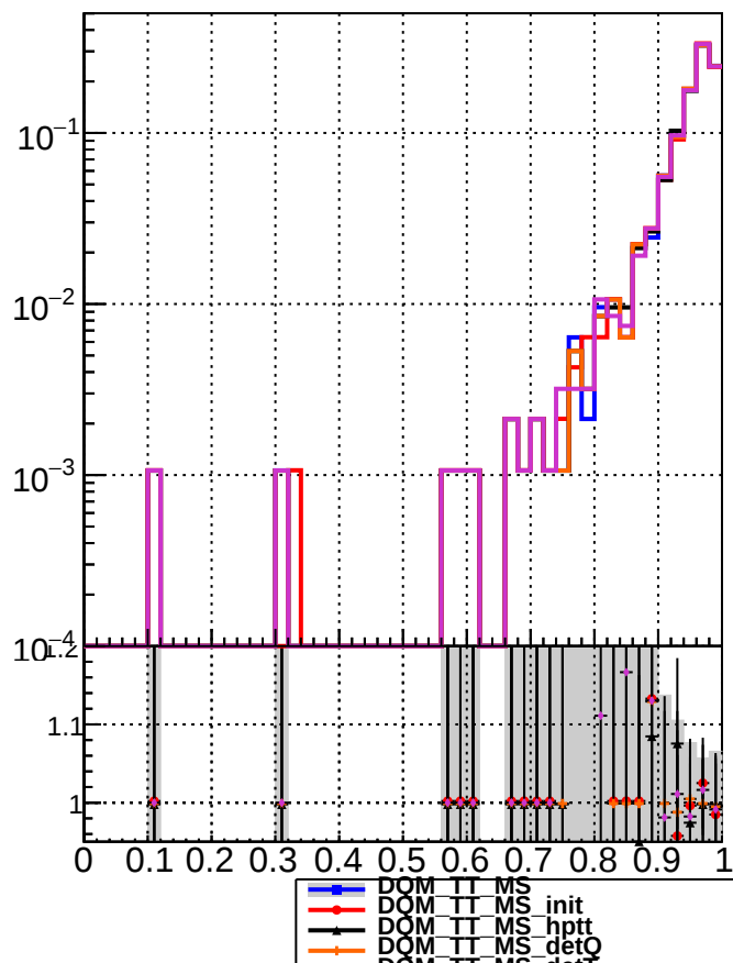
RecoPVAssoc2GenPVMatched_Missing
