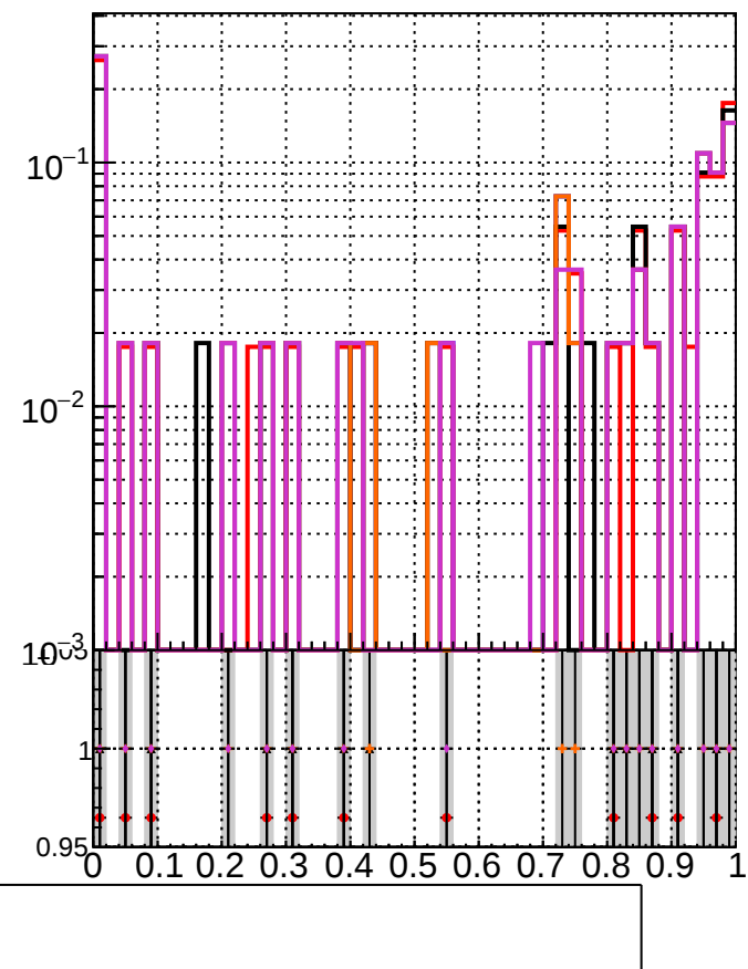
RecoPVAssoc2GenPVNotMatched_Missing
