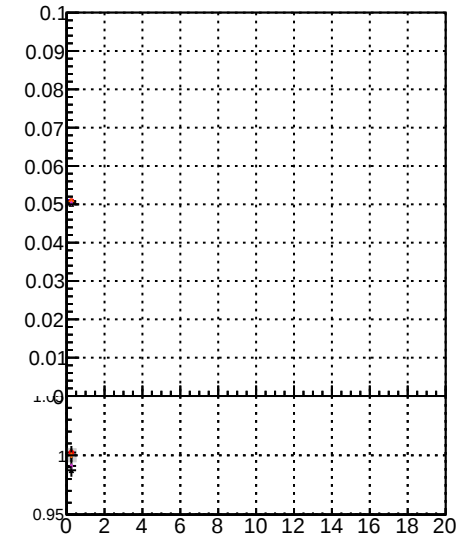
Fake rate vs. DOM TT MS and combinations
