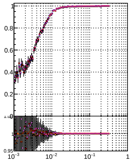
Fake rate vs \frac{dr}{pu}
