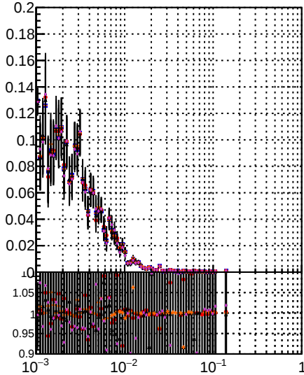
Duplicates Rate vs \frac{dr}{pu}
