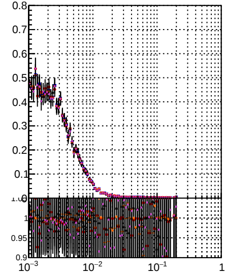
Pileup rate vs \frac{dr}{pu}
