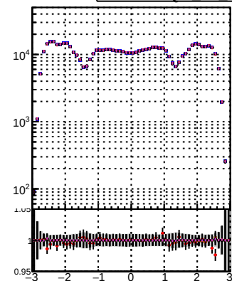
N of reco track vs e DOM TT MS hit 1 2 3 4 5 6 7 8 9 10
