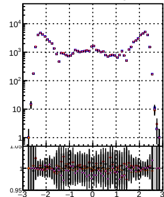
N of reco track vs \eta Legend: \frac{DQM}{QCD} , \frac{TT}{QCD} , \frac{MS}{QCD} , \frac{Unit}{QCD} , \frac{Data}{QCD}
