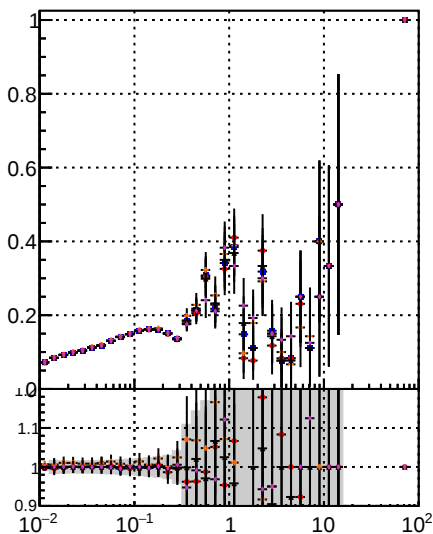
Fake rate vs \nu BQM TT MS init det
