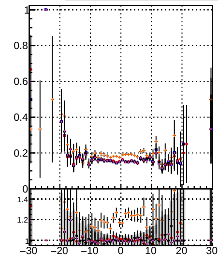
Fake rate vs v DOM TT MS init data mc
