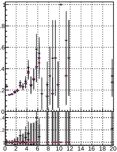
Fake rate vs. DOM TT MS DOM TT MS det
