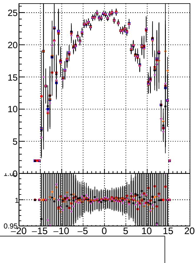
Reconstructed Tracks in Vertex (other Vtx) vs Z
