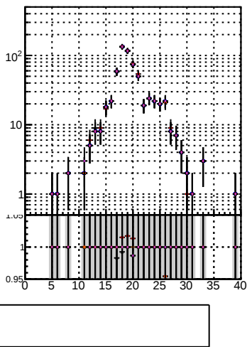
N of associated tracks (simToReco) vs hit
