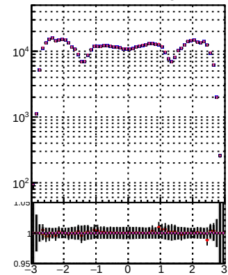
N of reco track vs \eta Legend: BQM, TT, MS, other
