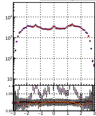
N of reco track vs \eta Legend: BQM, TT, MS, S, unit, det
