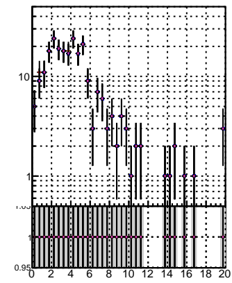
N of reco track vs. \chi^2 for different decay channels
