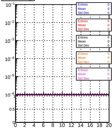
normalized \chi^2
