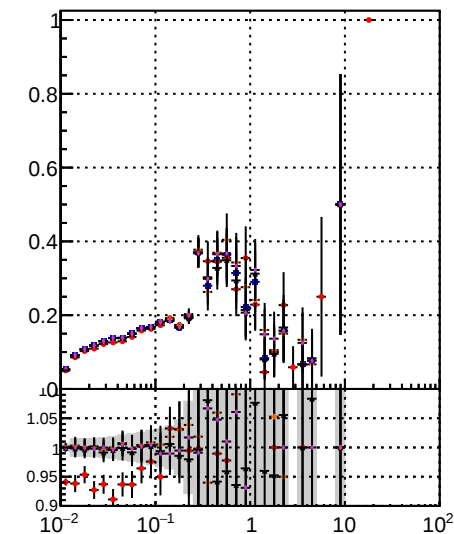
Fake rate vs v DOM TT MS init fake data
