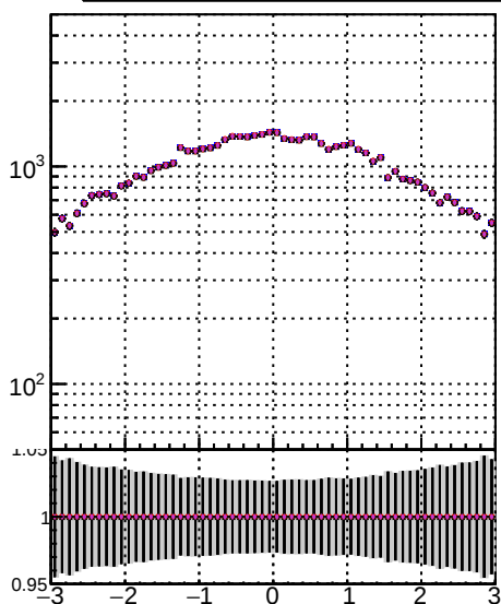
N of sim DOM TT MS hptt DOM TT MS hptt DOM TT MS detQ DOM TT MS detT
