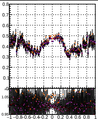
Legend DOM TT MS init det det Fake rate vs d ● ● ● ● ● ● Duplicates Rate vs Dxy(PV) ● ● ● ● ● ● Pileup rate vs dxy(PV) ● ● ● ● ● ●
