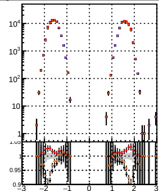
BGM RMS MS PL pixel-less model N of reco track vs \eta
