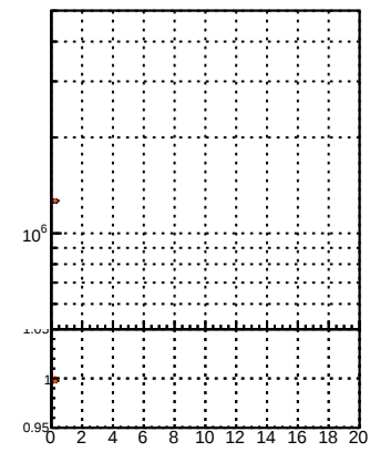
N of reco track vs. \chi^2 mod MS
