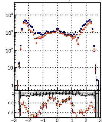
N of reco track vs \eta BGM RMS PL pixelLess RMS mod MS
