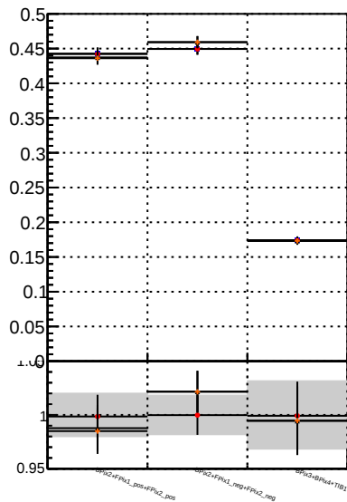
Fake rate vs. BQM noMS PL PixelLessOrandom mod MS
