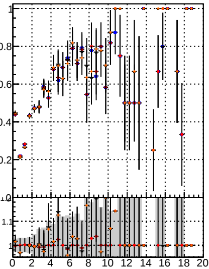
Fake rate vs. BQM noMS PL PixelLessOrandom mod MS
