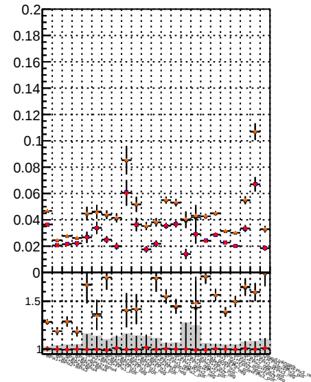
Fake rate vs. BQM, noMS, BQM, noMS, PL, PixelLessOrBQM mod MS
