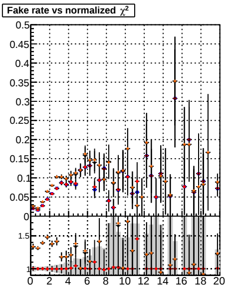
Fake rate vs. BQM, noMS, BQM, noMS, PL, PixelLessOrBQM mod MS
