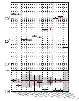
N of reco track vs. \chi^2 mod MS
