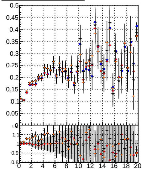
Fake rate vs. BQM pMS PLMS pixelLessOrpBQM mod MS
