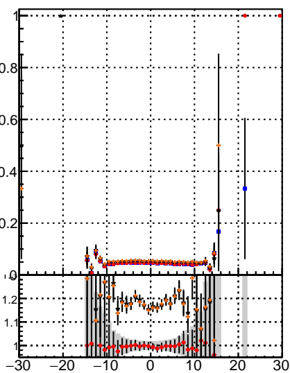
Fake rate vs dxy —●— DCM mod MS —●— DCM mod MS PLMS —●— DCM mod MS PLMS —●— DCM mod MS PLMS
