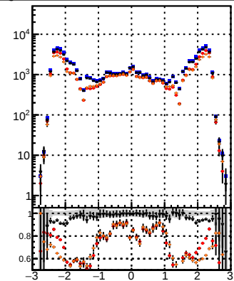
N of reco track vs \eta BGM RMS MS PL pixelLess BGM mod MS
