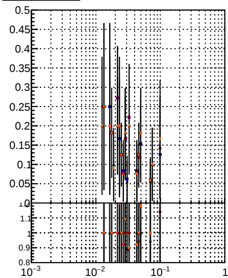
Fake rate vs \frac{DOM_{noMS}}{DOM_{MS\_PL}} \frac{Orig/DOM\_orig\_MS}{pixelLessOrig/DOM\_mod\_MS}
