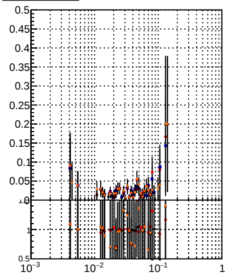
Fake rate vs dr Legend: DOM no MS (blue squares) DOM MS PL (red circles) Orig/DOM orig MS (black circles) pixelLessOrig/DOM mod MS (orange circles)
