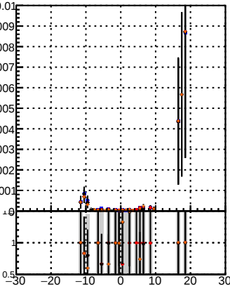
Duplicates Rate vs Dz(PV)
