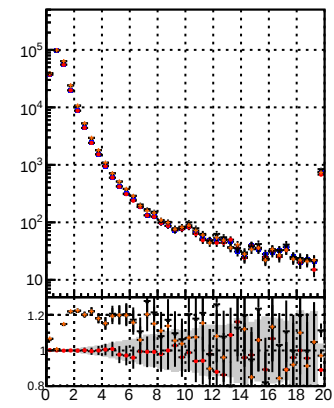
N of reco track vs. \chi^2 BOM reMS BOM reMS PL BOM reMS PL MS pixelLess reMS pixelLess reMS mod MS
