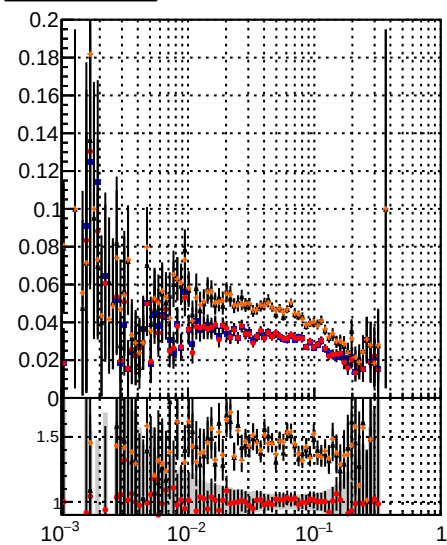
Fake rate vs \mu Legend: DOM noMS (black line) DOM MS PL (blue line) orig/DOM orig MS (red line) pixelLessOrig/DOM mod MS (orange line)
