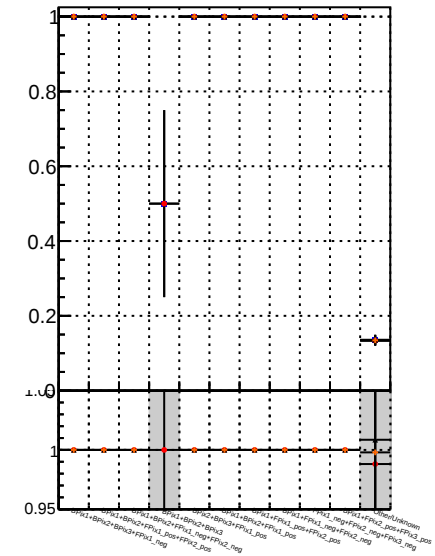
Fake rate vs. BQM pBMS PL pixelLess BQM mod MS
