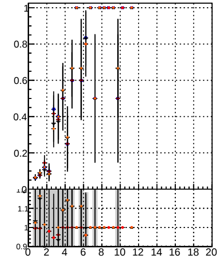
Fake rate vs. BQM pBMS PL pixelLess BQM mod MS
