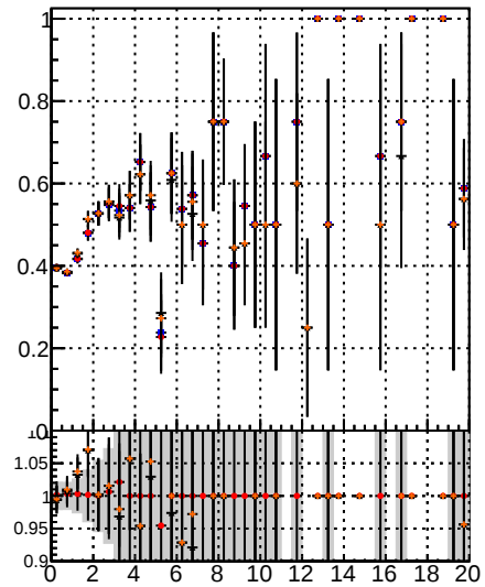
Fake rate vs. BQM noMS BQM noMS PL PixelLessOrandom BQM mod MS
