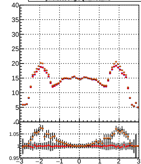
mean hit Legend: DQM_noMS (blue line), DQM_noMS_PL (red line), Orig/DQM_orig_MS (black line), pixelLessOrig/DQM_mod_MS (orange line)
