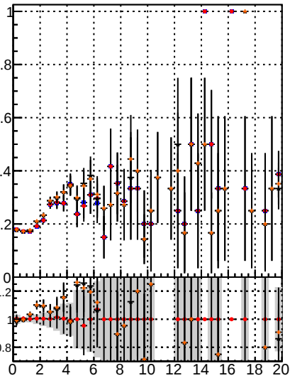
Fake rate vs. BQM noMS BQM noMS PL PixelLessOrNoBQM BQM mod MS
