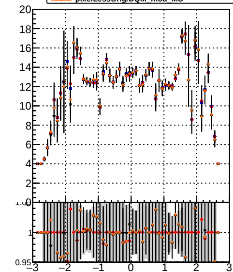
mean hit Legend: DQM_noMS (blue line with circles), DQM_moMS_PL (red line with circles), Orig/DQM_orig_MS (black line with circles), pixelLessOrig/DQM_mod_MS (orange line with circles)
