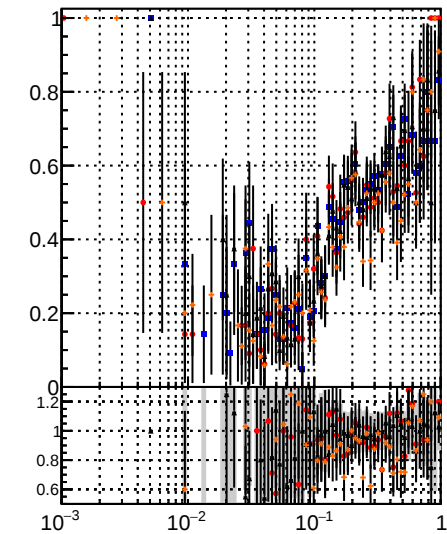
Fake rate vs dr Legend: DOM noMS (blue squares) DOM MS PL (red circles) Orig/DOM orig MS (black triangles) pixelLessOrig/DOM mod MS (orange triangles)
