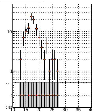
N of reco track vs hit DOM noMS DOM modMS_PL origDOM orig MS pixelLessOrigDOM mod MS
