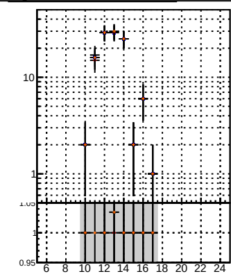
N of reco track vs hit DOM noMS DOM modMS_PL origDOM orig MS pixelLessOrigDOM mod MS
