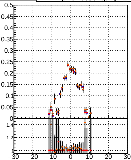
Fake rate vs v Legend: DOM noMS DOM noMS PL Orig/DOM orig MS pixelLessOrig/DOM mod MS
