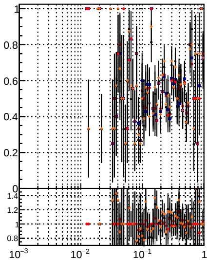
Fake rate vs \mu Legend: DOM noMS (black line) DOM MS PL (blue line) Orig/DOM orig MS (red line) pixelLessOrig/DOM mod MS (orange line)
