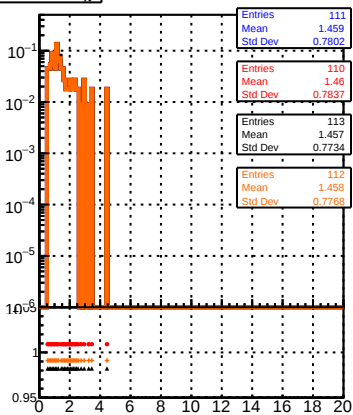
normalized \chi^2
