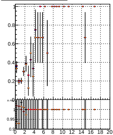
Fake rate vs. BQM noMS BQM noMS PL OLS PL pixelLess noBQM mod MS
