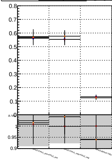
Fake rate vs. BQM noMS BQM noMS PL OLS PL pixelLess noBQM mod MS
