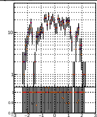
N of reco track vs \eta BSM mod MS, PL, pixelLessOrigMS
