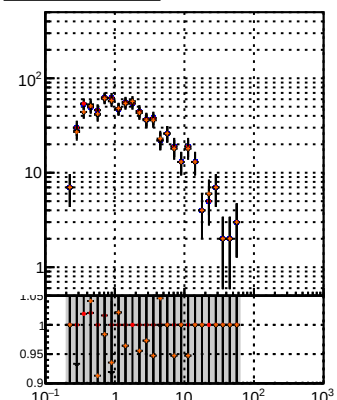
N of reco track vs \eta BSM mod MS, PL, pixelLessOrigMS
