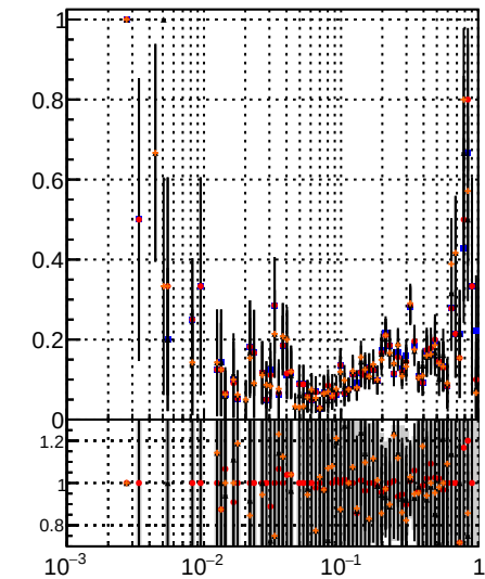
Fake rate vs dr Legend: DOM noMS (blue squares) DOM MS PL (red circles) Orig/DOM orig MS (black triangles) pixelLessOrig/DOM mod MS (orange crosses)
