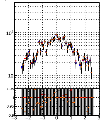
N of reco track vs \eta BSM MS PL pixelLess N of associated (recoToSim) tracks vs \eta BSM MS PL pixelLess N of associated (recoToSim) duplicate tracks vs \eta BSM MS PL pixelLess
